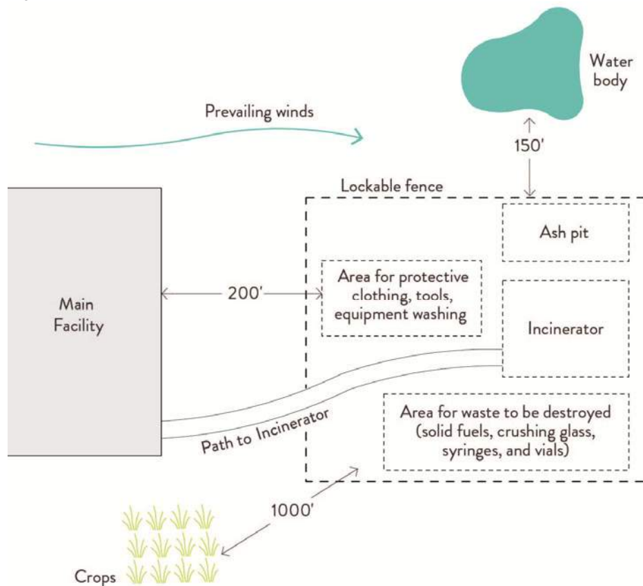
Figure 29.e. Incinerator area
