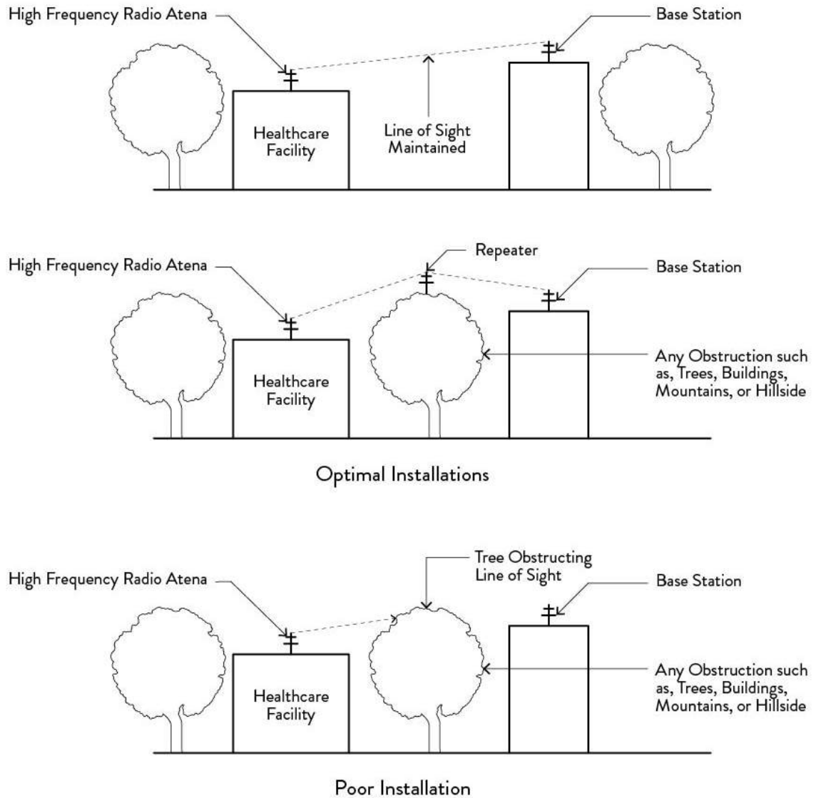
Figure 26.a. Recommended HF Radio Installation
