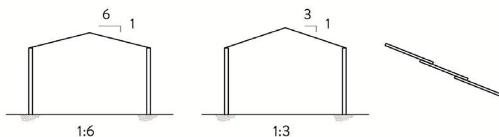
Figure 36.a. Roof Slope
