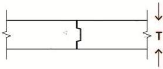
Figure 39.d. Concrete Key
