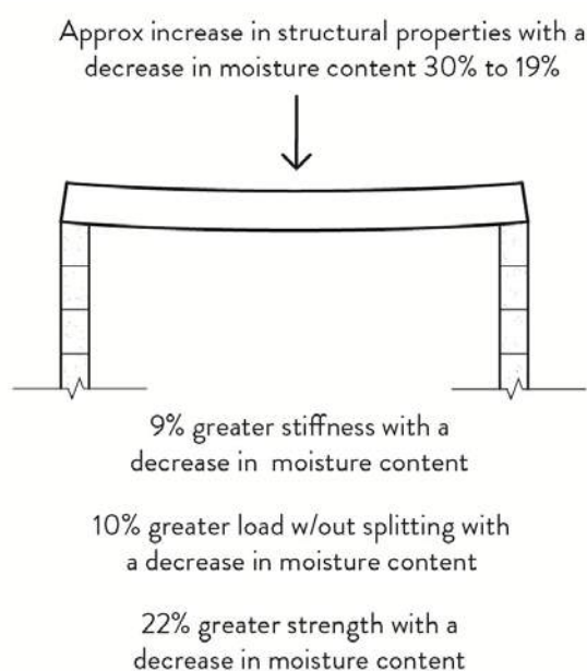
Figure 43.a. Moisture Content Effects
