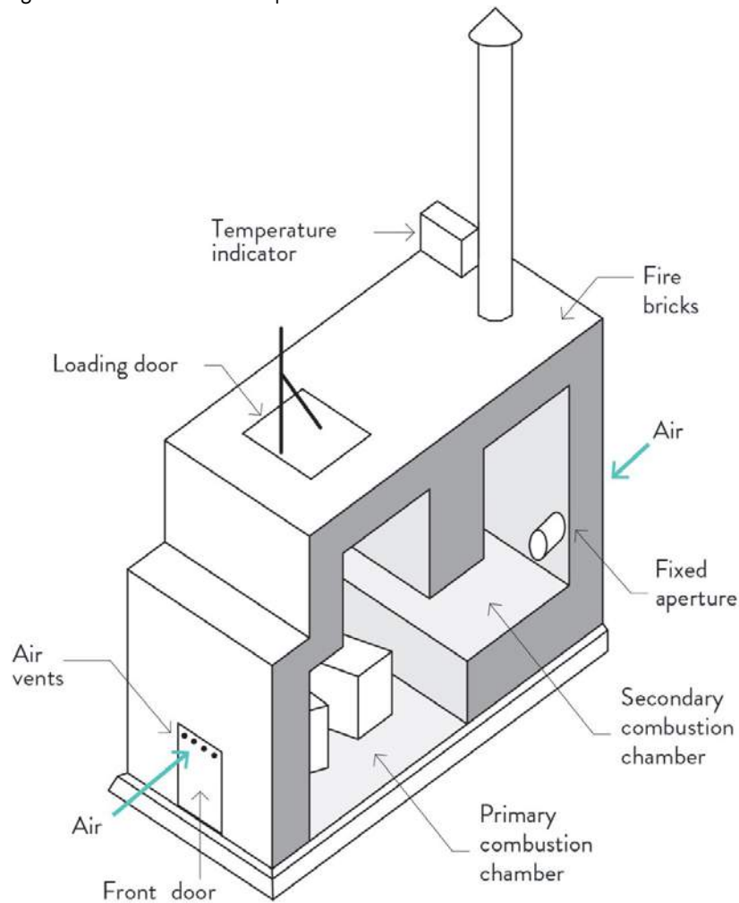
Figure 29.f. Incinerator components
