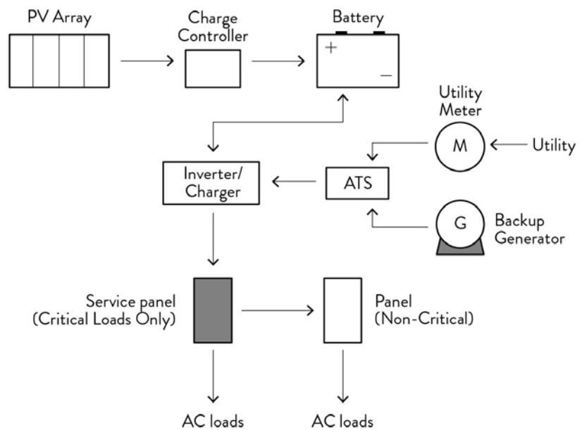
Figure 23.b Generator/Utility/Grid-Tied PV with Batteries
