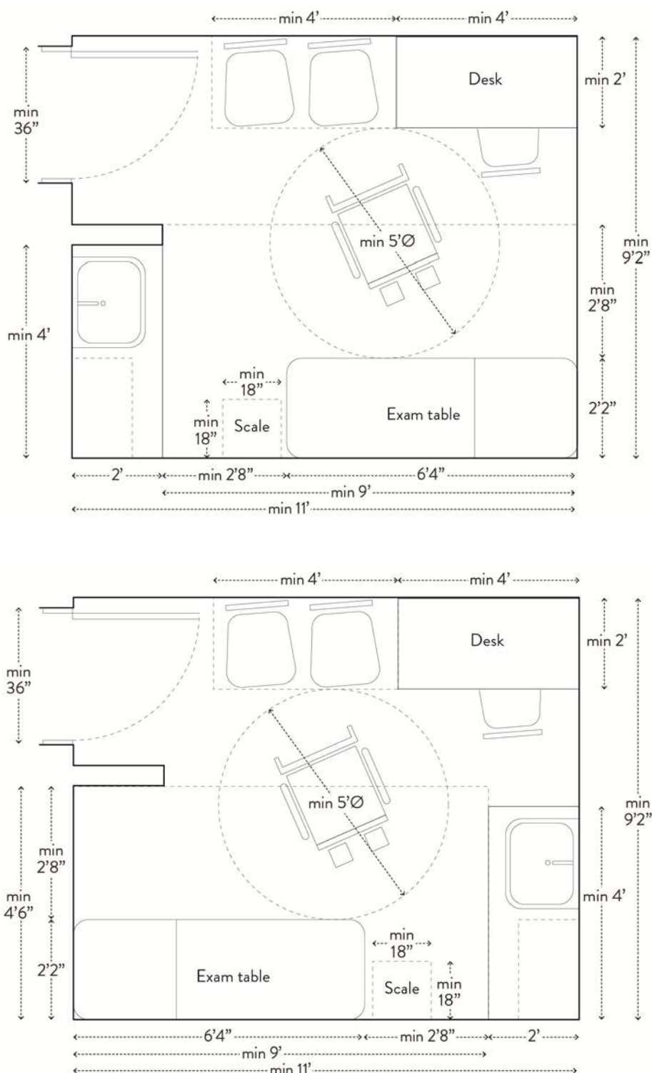
Figure 48.a. Possible Consultation Room Layouts.
