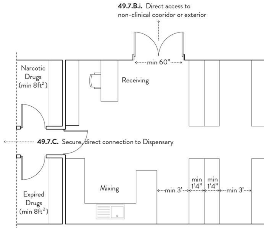
Figure 49.d. Pharmacy Stock Requirements and Possible Layout
