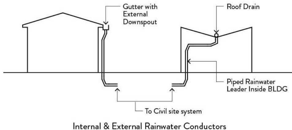
Figure 30.i. Examples of internal roof drainage
