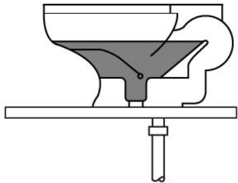
Figure 30.f. Fixture with integral trap
