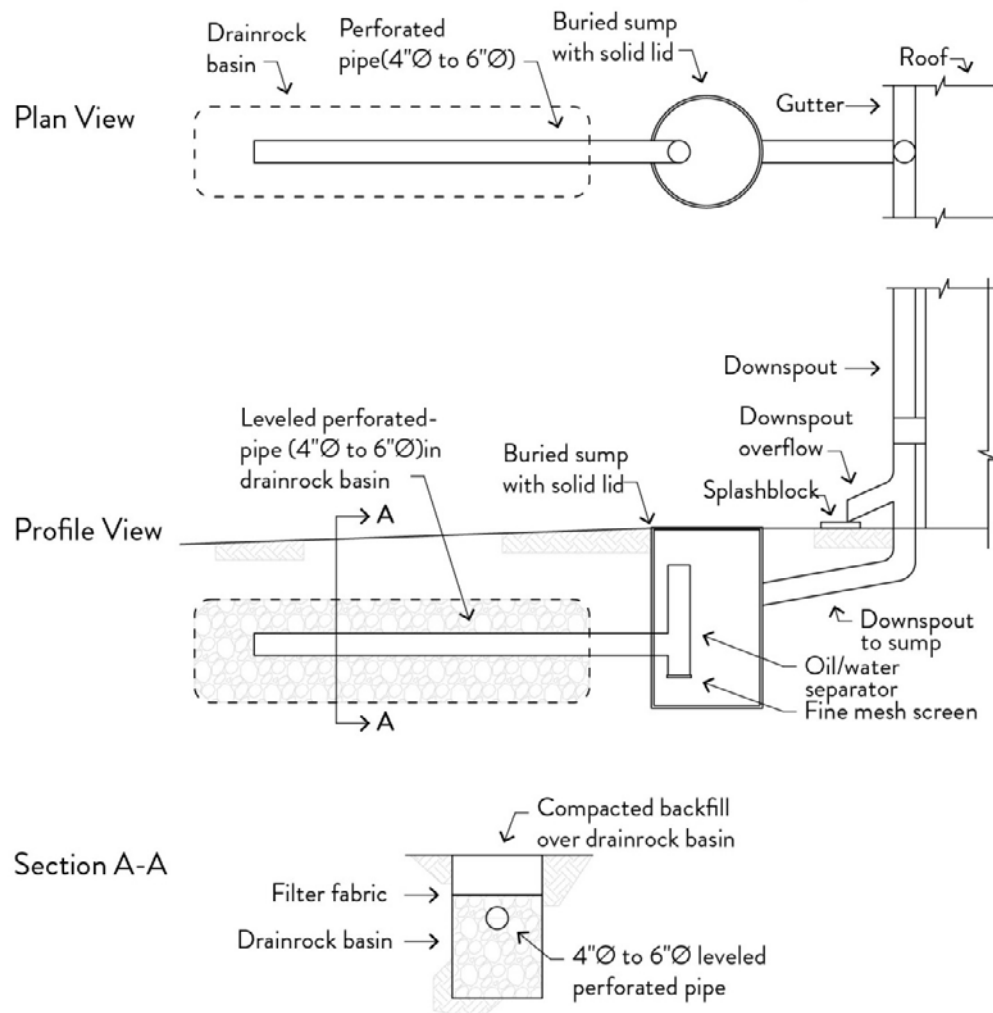
Figure 11.a. Typical Downspout Infiltration System
