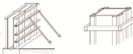
Figure 39.b Formwork Layout
