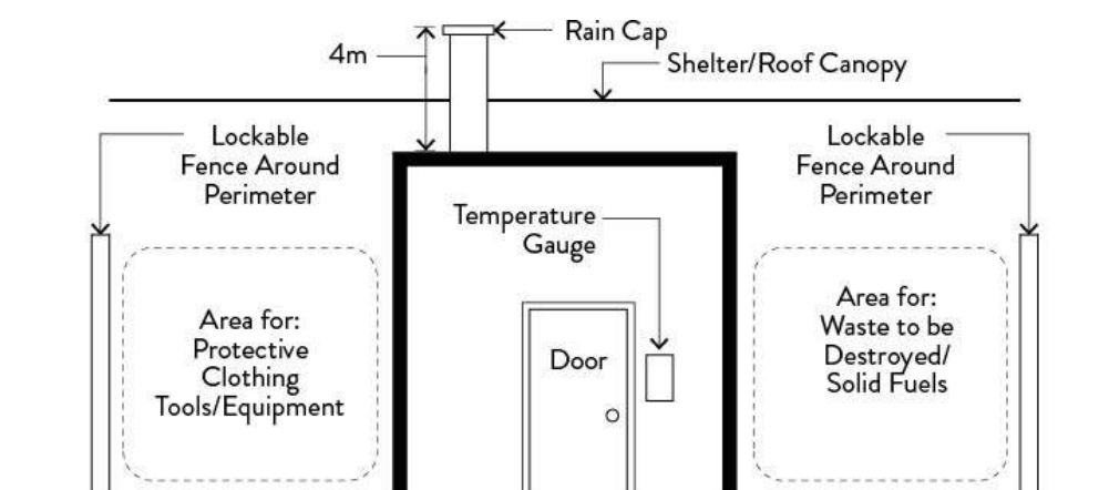
Figure 29.d. Example Incinerator
