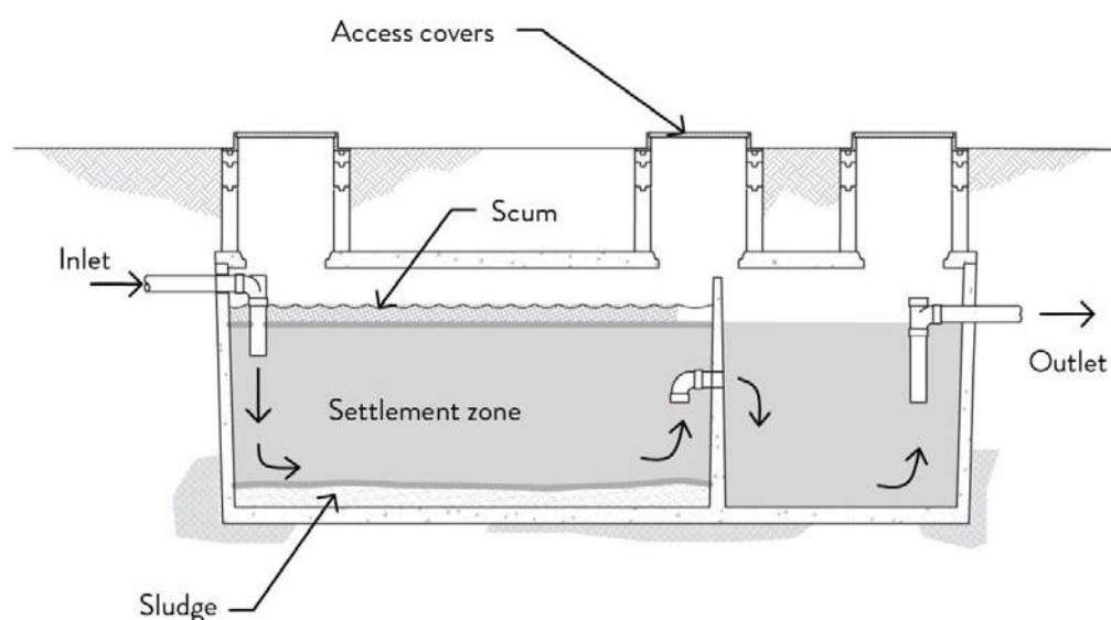
Figure 28.e. Septic Tank
