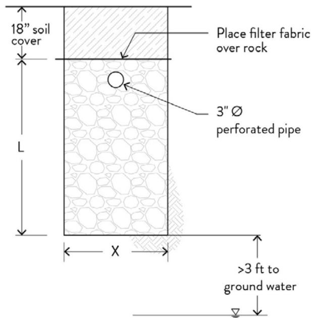
Figure 29.o. Subsurface Disposal System Sizing
