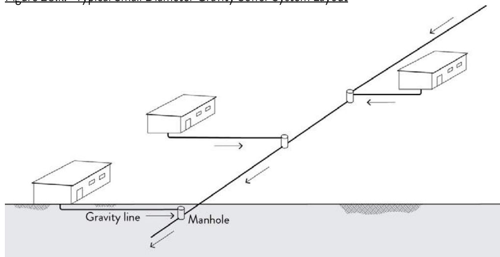
Figure 28.k. Typical Small Diameter Gravity Sewer System Layout
