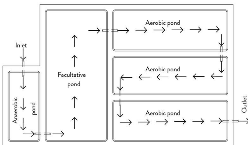
Figure 28.j. Waste Stabilization Pond Layout
