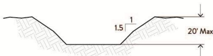
Figure 33.e. Excavation
