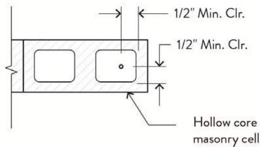
Figure 40.c.Reinforcement Placement Requirements
