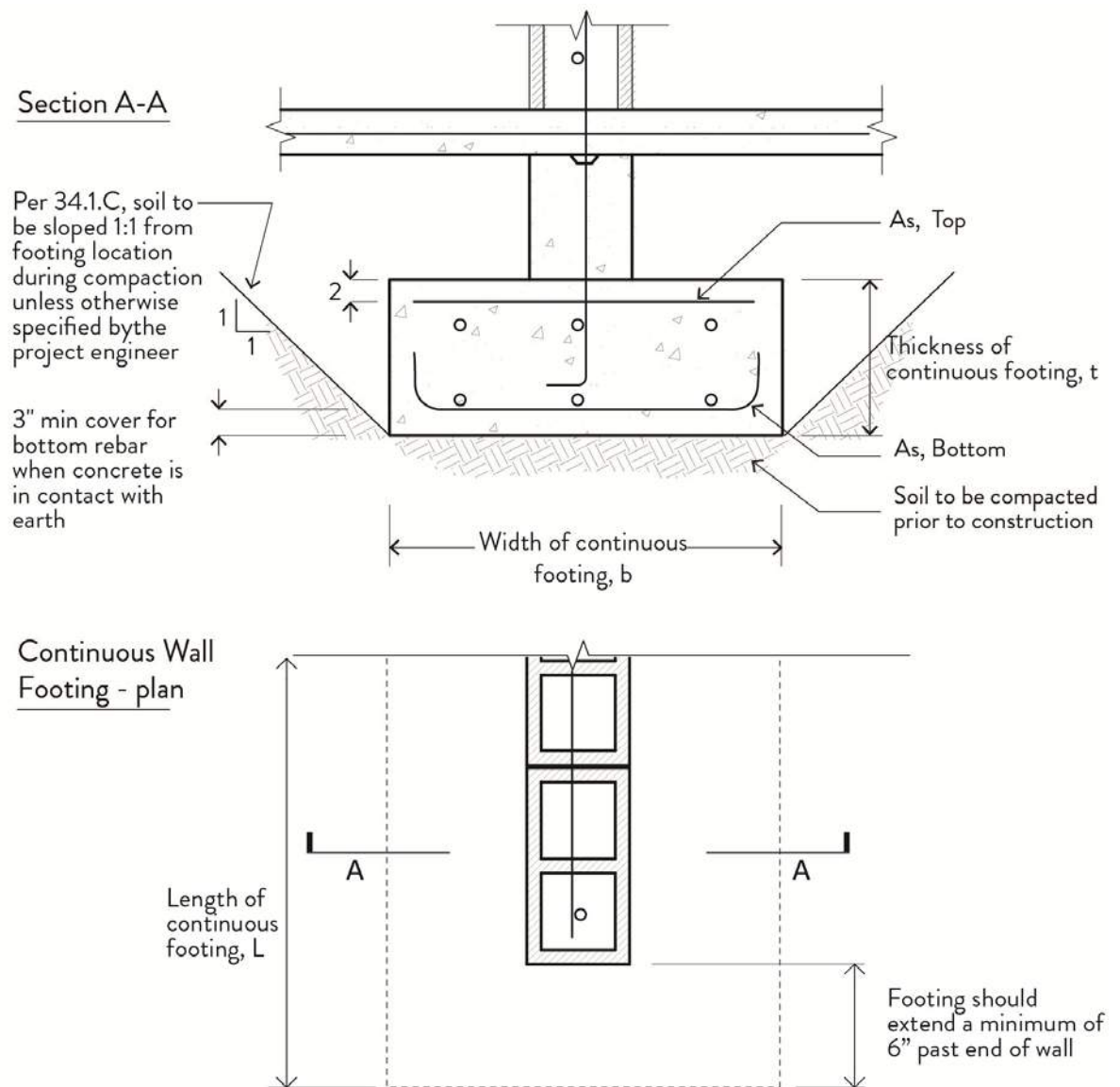
Figure 34.c. Continuous Foundation Detail Example - Type 1
