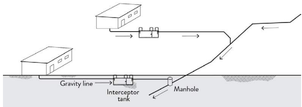
Figure 28.l. Typical Small Diameter Gravity Effluent Sewers with Interceptor (Septic) Tanks Before Sewers
