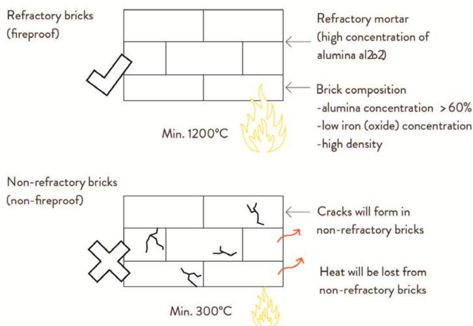
Figure 29.g. Refractory vs. Non-refractory bricks
