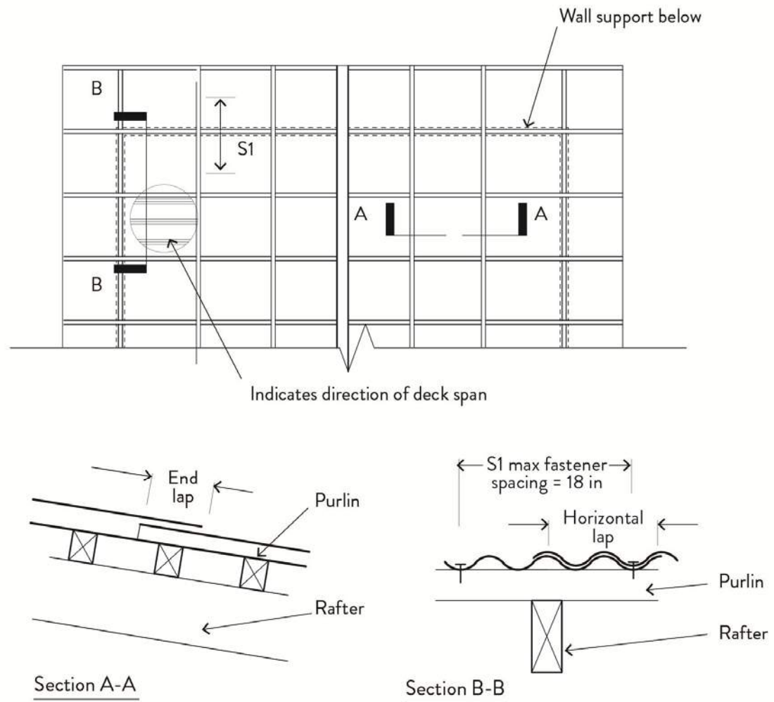
Figure 36.b. Roof Deck Attachment Detail (Wood Framing)
