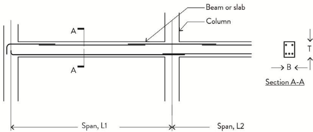
Figure 36.j. Concrete Beam and Slab Span
