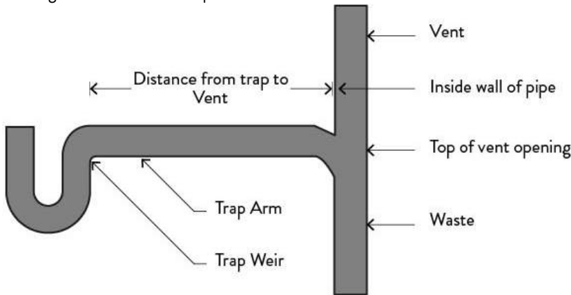
Figure 30.g. Distance from Trap to Vent
