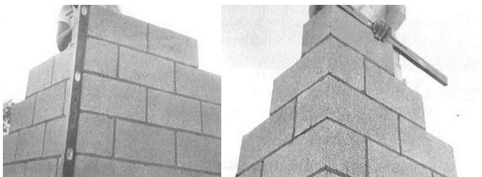
Figure 40.b. Typical Corner Construction
