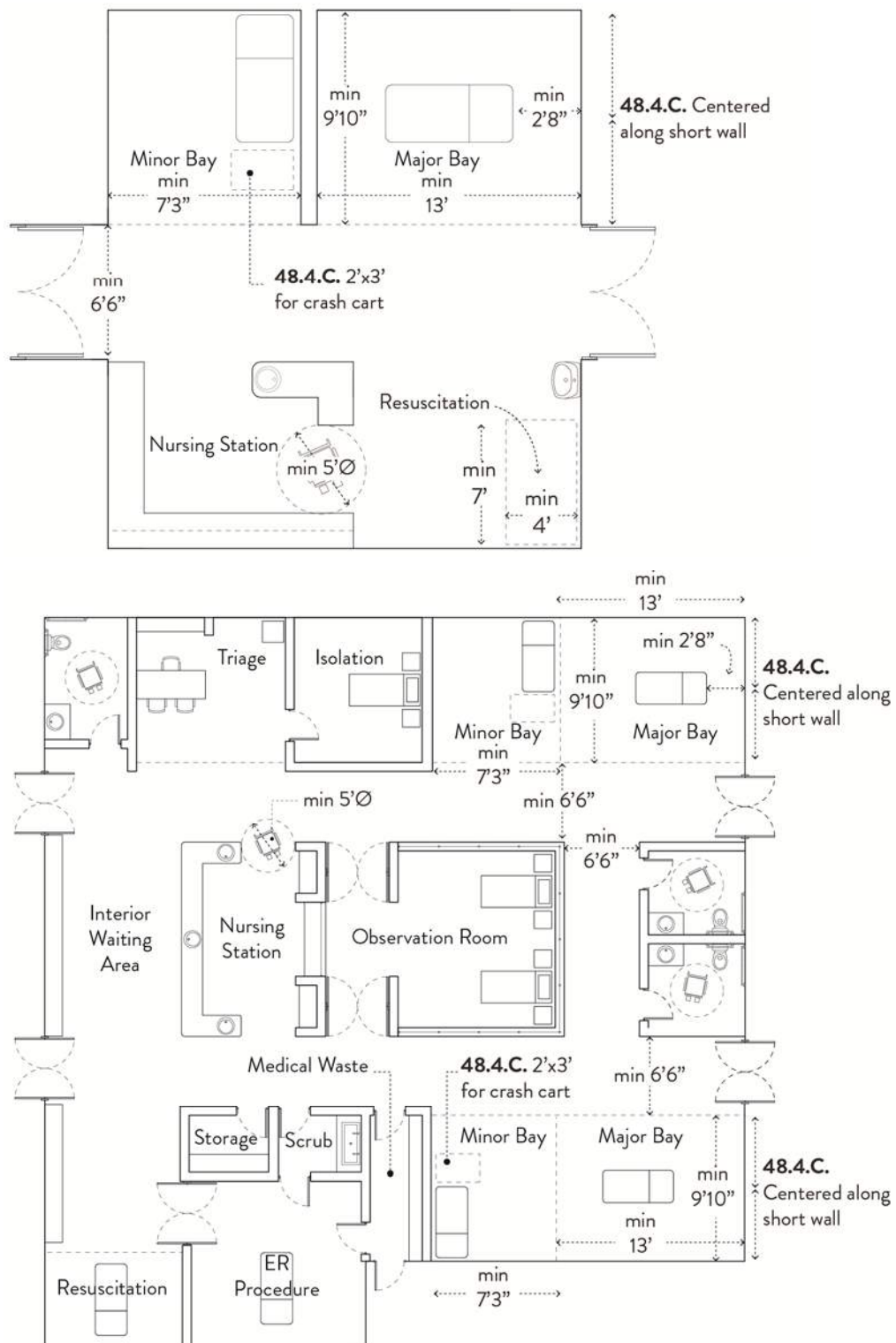
Figure 48.d. Possible Large and Small ER Layouts.
