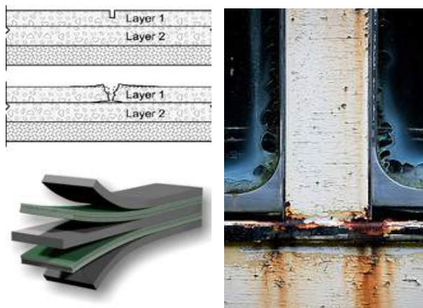
Figure 41.a.Steel Delamination
