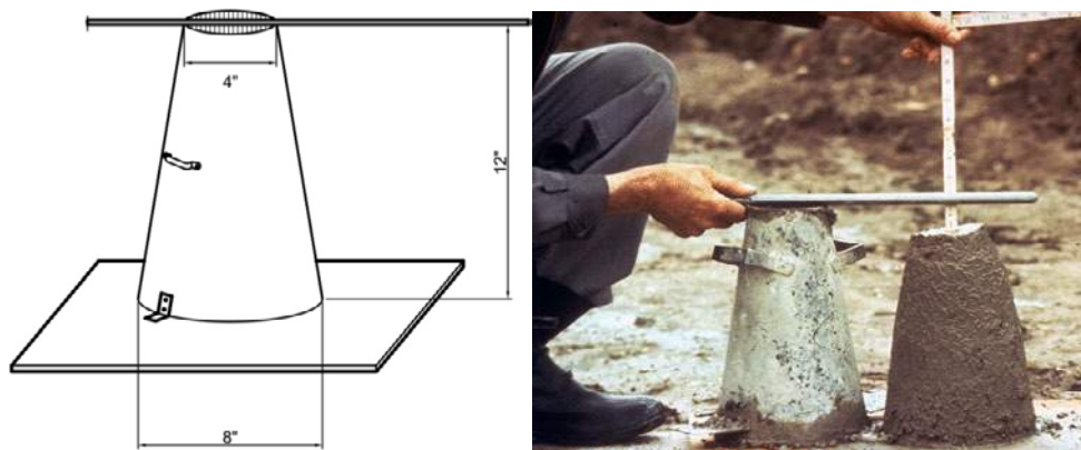
Figure 39.a.Slump “Cone” Parameters (left); Slump Test Example (right)
