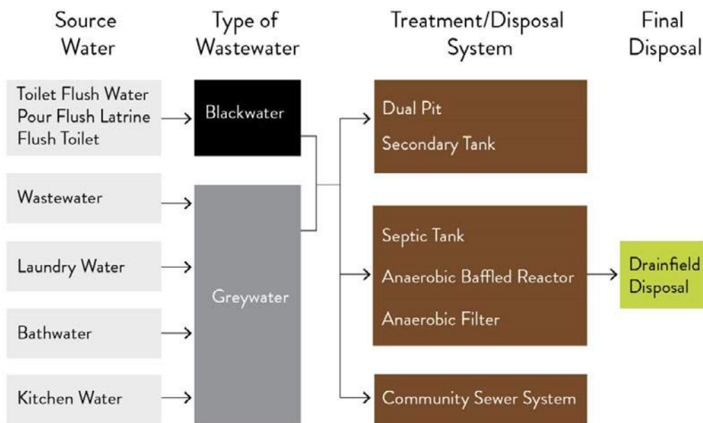
Figure 28.b. Wet Sanitation System Types
