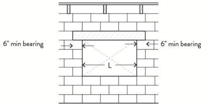
Figure 40.f.Lintel Construction
