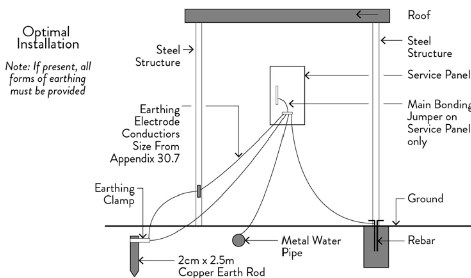
Figure 23.h. Key elements in earthing systems
